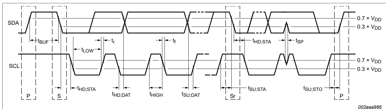
Figure 18. Definition of timing on the I 2 C-bus
