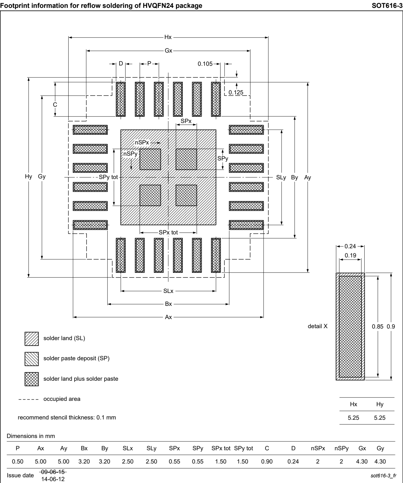
Figure 25. PCB footprint for SOT616-3 (HVQFN24); reflow soldering
