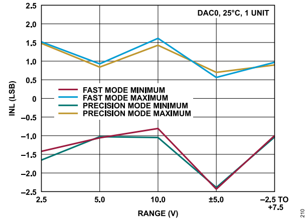
Figure 19. INL vs. Range, Fast Mode and Precision Mode
