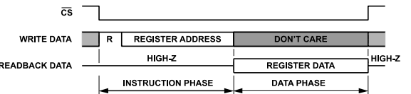
Figure 72. Basic SPI Read Frame
