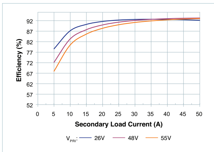
Figure 3 — Efficiency at -40^\circ\text{C}
