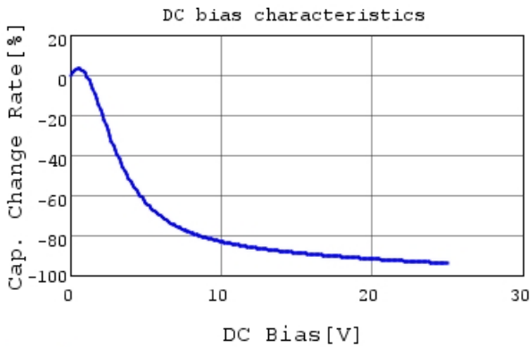
GRM155R61E105MA12 C-DC bias capchange, 25.0c
