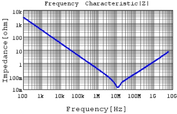
GRM155R61E105MA12 |Z| DCOV,25degC
