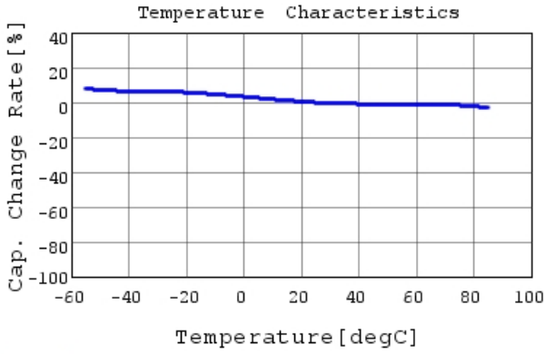
GRM155R61E105MA12 C-Temp. capchange, DC0.0V,
