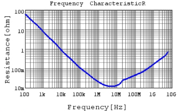
GRM155R61E105MA12 R DCOV,25degC
