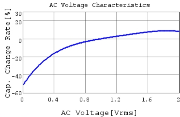
GRM155R61E105MA12 C-AC Voltage capchange, DC
