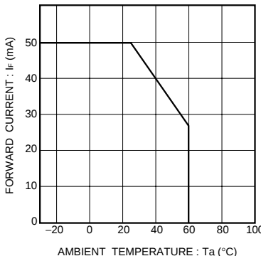
Fig.7 Forward current falloff
