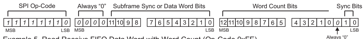
FIGURE 5. ARINC 717 & SPI Bit Ordering
