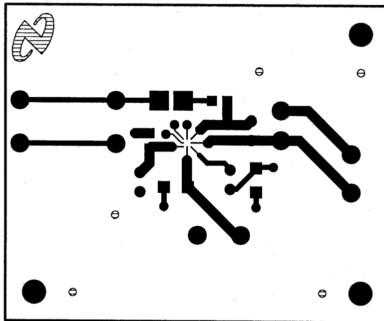
Figure 41. Top Layer
