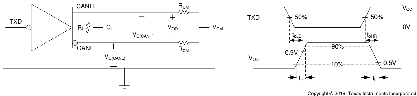
Figure 7-1. Driver Test Circuit and Measurement
