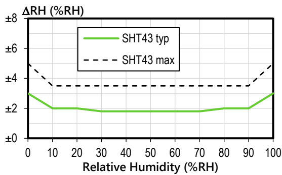
Figure 4. SHT43 typical and maximal relative humidity accuracy at 25 °C.
