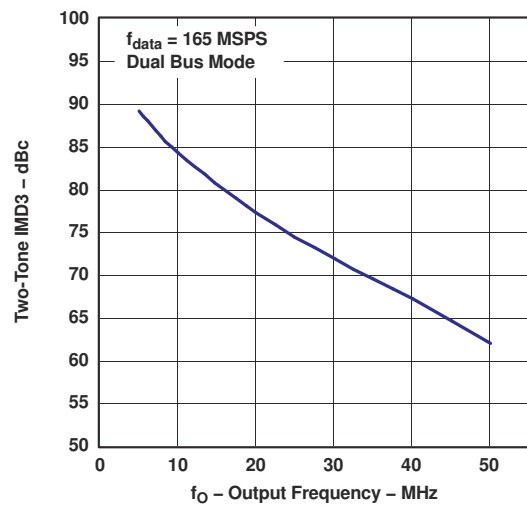
Figure 6-10. Two-Tone IMD3 vs Output Frequency
