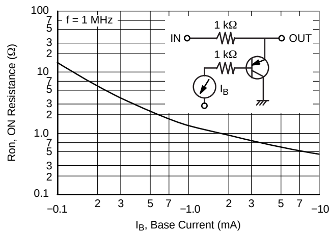
Figure 10. R_{on} - I_B
