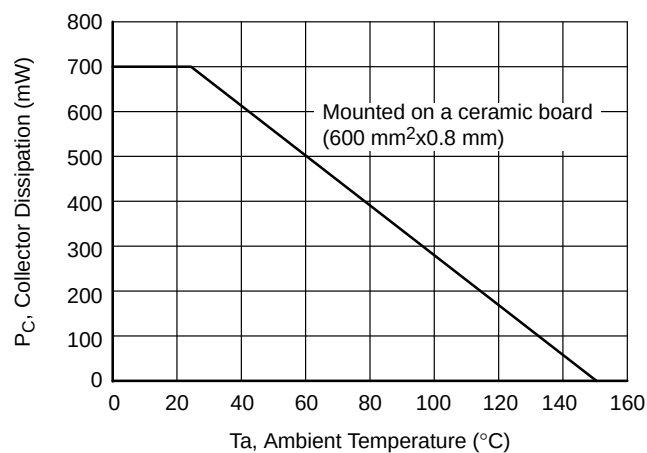
Figure 11. P_C - T_a
