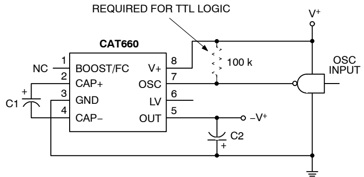
Figure 17. External Clocking
