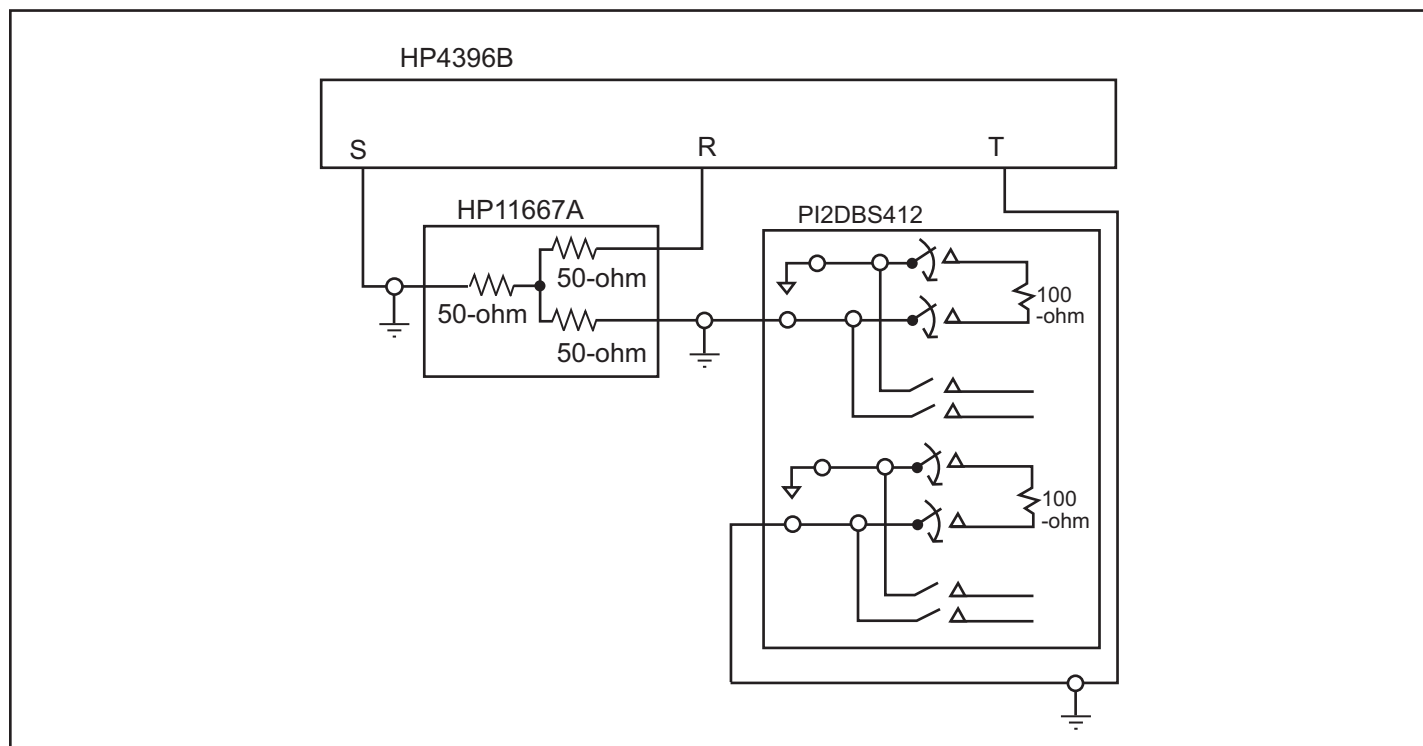
Fig 1. Crosstalk Setup
