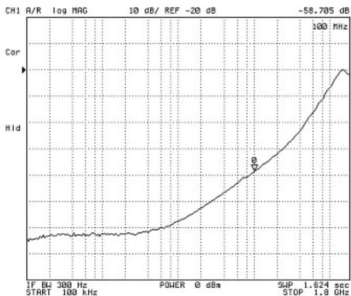
Fig 5. Off Isolation
