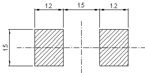
Recommend Soldering Pad
