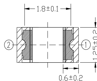
Recommend Soldering Pad
