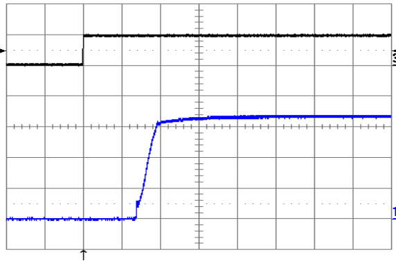
Figure 17. Turn-on transient at full rated load current (resistive) with no out-put capacitor at V_{in} = 48\text{ V} , triggered via ON/OFF pin. Top trace: ON/OFF signal (5 V/div.). Bottom trace: output voltage (1 V/div.). Time scale: 1 ms/div.
