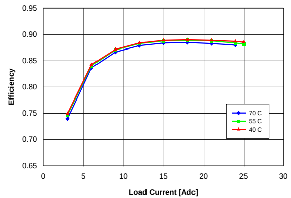
Figure 14. Efficiency vs. load current and ambient temperature for converter mounted vertically with V_{in} = 54\text{ V} and air flowing from pin 3 to pin 1 at a rate of 200 LFM (1.0 m/s).
