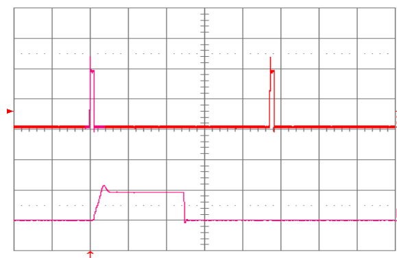
Figure 26. Load current (top trace, 20 A/div, 20 ms/div) into a 10 mΩ short circuit during restart, at Vin = 48 V. Bottom trace (40 A/div, 1 ms/div) is an expansion of the on-time portion of the top trace.
