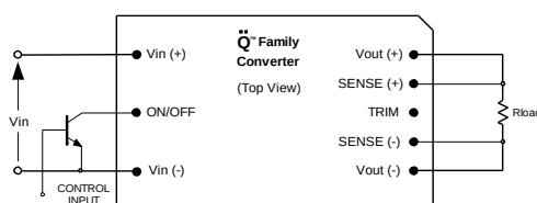
Figure 1. Circuit configuration for ON/OFF function.
