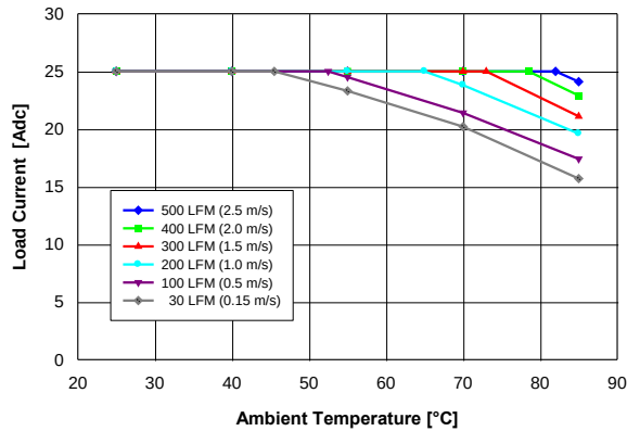
Figure 9. Available load current vs. ambient air temperature and airflow rates for converter mounted vertically with V_{in} = 54 V, air flowing from pin 3 to pin 1 and maximum FET temperature \leq 120 °C
