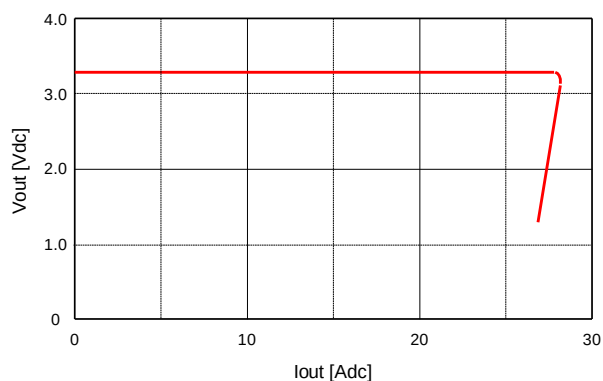
Figure 25. Output voltage vs. load current showing current limit point and converter shutdown point. Input voltage has almost no effect on current limit characteristic.
