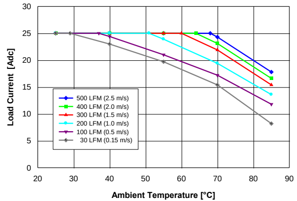
Figure 10. Available load current vs. ambient air temperature and airflow rates for converter mounted vertically with V_{in} = 54 V, air flowing from pin 3 to pin 1 and maximum FET temperature \leq 105 °C.
