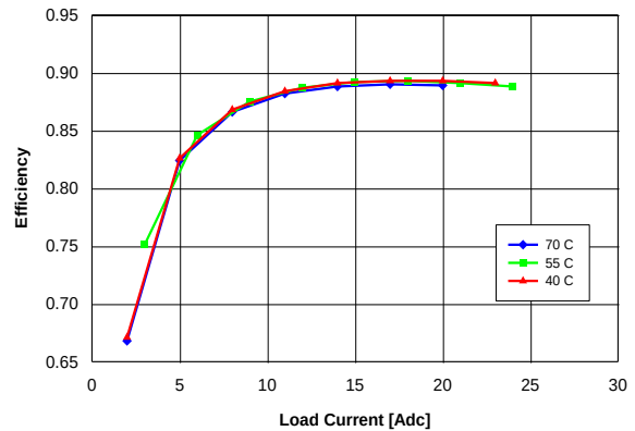
Figure 16. Efficiency vs. load current and ambient temperature for converter mounted horizontally with V_{in} = 54\text{ V} and air flowing from pin 3 to pin 4 at a rate of 200 LFM (1.0 m/s).
