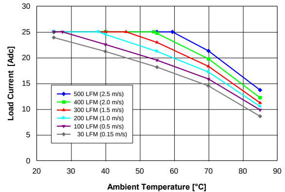
Figure 12. Available load current vs. ambient temperature and airflow rates for converter mounted horizontally with V_{in} = 54 V, air flowing from pin 3 to pin 4 and maximum FET temperature \leq 105 °C
