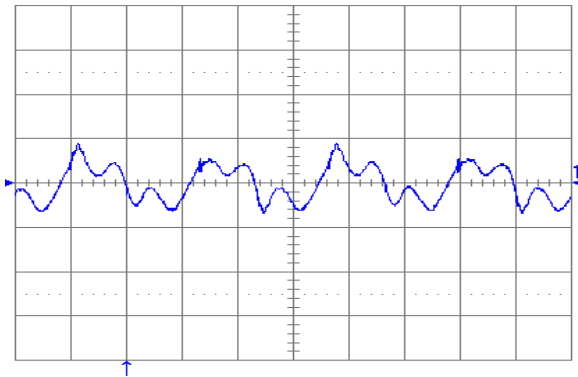
Figure 21. Output voltage ripple (20 mV/div.) at full rated load current into a resistive load with C_o = 10 \mu F tantalum + 1 \mu F ceramic and V_{in} = 48 V. Time scale: 1 \mu s/div.
