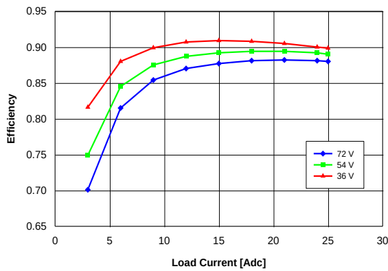
Figure 15. Efficiency vs. load current and input voltage for converter mounted horizontally with air flowing from pin 3 to pin 4 at a rate of 300 LFM (1.5 m/s) and T_a = 25^\circ\text{C} .
