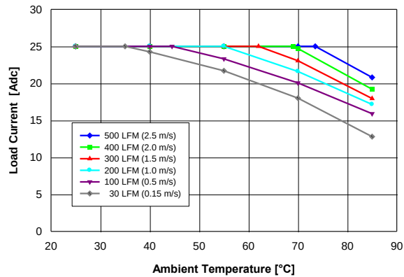
Figure 11. Available load current vs. ambient temperature and airflow rates for converter mounted horizontally with V_{in} = 54 V, air flowing from pin 3 to pin 4 and maximum FET temperature \leq 120 °C.
