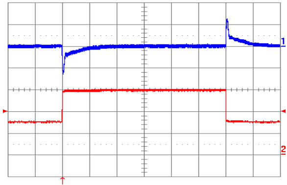
Figure 20. Output voltage response to load current step-change (7.5 A – 15 A – 7.5 A) at V_{in} = 48 V. Top trace: output voltage (100 mV/div). Bottom trace: load current (5 A/div). Current slew rate: 5 A/ \mu s. C_o = 450 \mu F tantalum + 1 \mu F ceramic. Time scale: 0.2 ms/d
