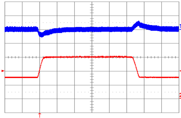
Figure 19. Output voltage response to load current step-change (7.5 A – 15 A – 7.5 A) at V_{in} = 48 V. Top trace: output voltage (100 mV/div). Bottom trace: load current (5 A/div). Current slew rate: 0.1 A/ \mu s. C_o = 1 \mu F ceramic. Time scale: 0.2 ms/div..
