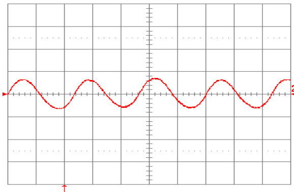
Figure 23. Input reflected ripple current, i_c (100 mA/div), measured at input terminals at full rated load current and V_{in} = 48 V. Refer to Fig. 22 for test setup. Time scale: 1 \mu s/div.
