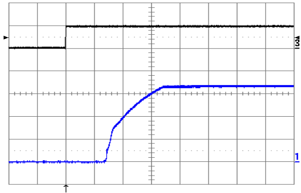
Figure 18. Turn-on transient at full rated load current (resistive) plus 10,000 \mu\text{F} at V_{in} = 48\text{ V} , triggered via ON/OFF pin. Top trace: ON/OFF signal (5 V/div.). Bottom trace: output voltage (1 V/div.). Time scale: 1 ms/div.
