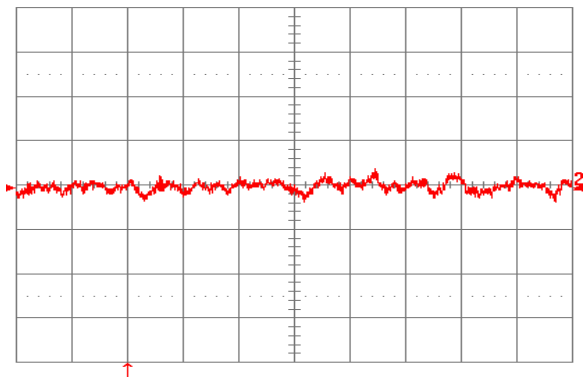
Figure 24. Input reflected ripple current, i_s (10 mA/div), measured through 10 \mu H at the source at full rated load current and V_{in} = 48 V. Refer to Fig. 22 for test setup. Time scale: 1 \mu s/div.
