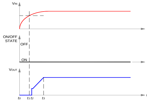
Figure 6. Start-up scenario #1.
