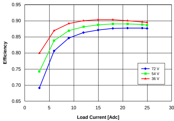
Figure 13. Efficiency vs. load current and input voltage for converter mounted vertically with air flowing from pin 3 to pin 1 at a rate of 300 LFM (1.5 m/s) and T_a = 25^\circ\text{C} .
