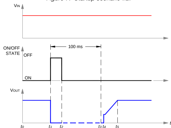
Figure 8. Startup scenario #3.
