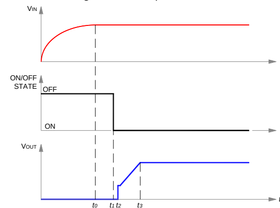
Figure 7. Startup scenario #2.
