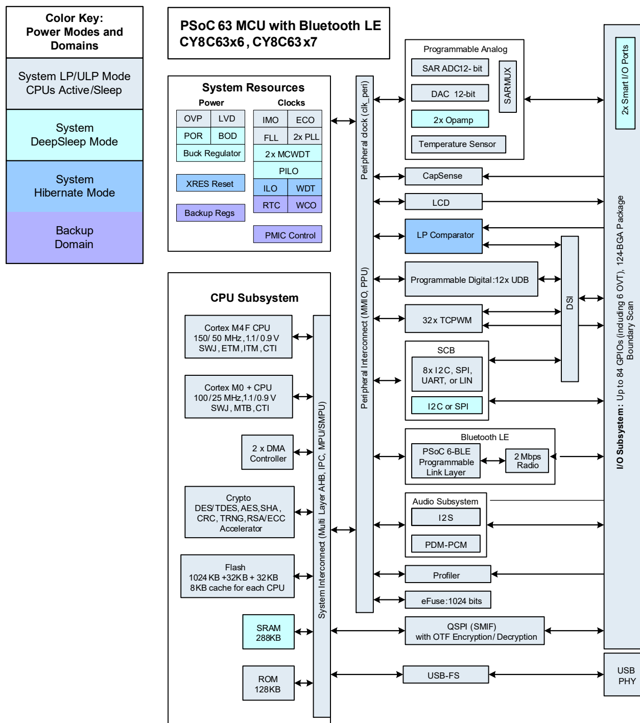
Figure 3. Block Diagram
