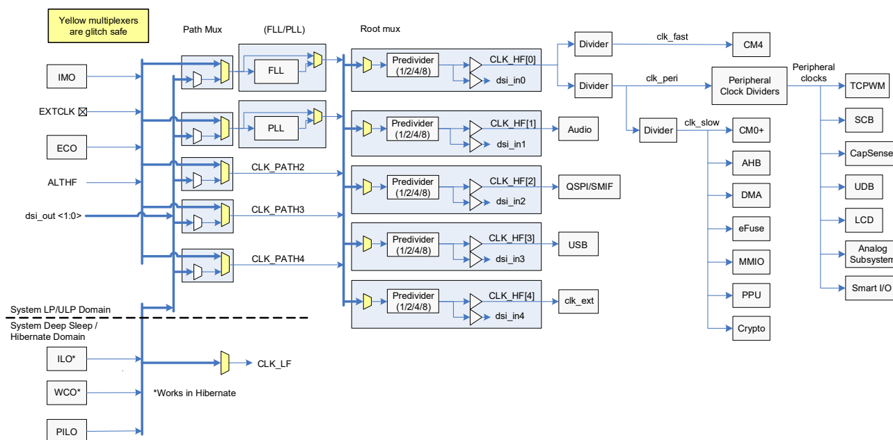
Figure 4. Clocking Diagram
