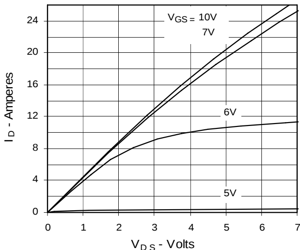
Fig. 1. Output Characteristics @ 25^\circ\text{C}
