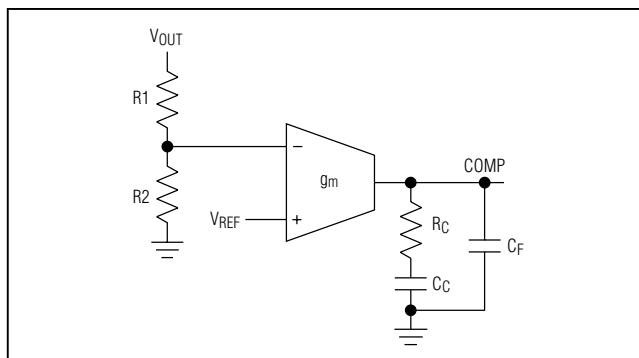
Figure 4. Compensation Network
