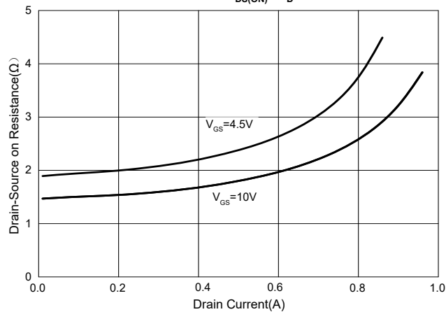
Fig. 4 - R_{DS(ON)} vs I_D
