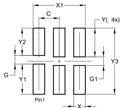
X1-DFN1010-6 (Type B)
