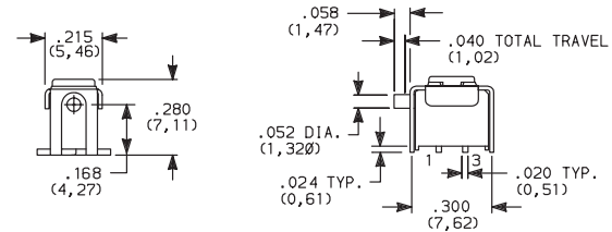
GP11MSV1BE SPST
