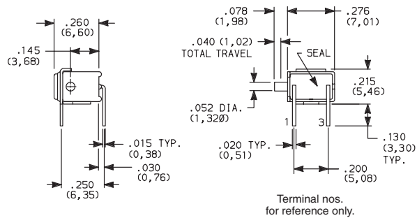
GP11MABE SPST
