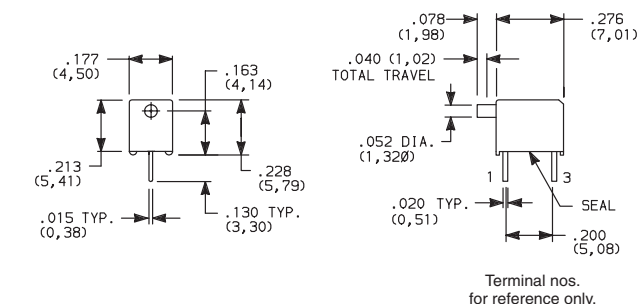
GP11MCBE SPST
