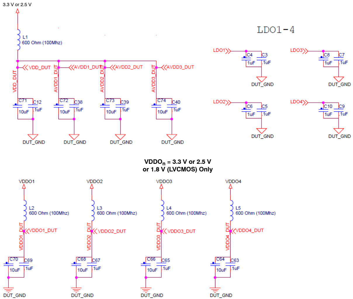
Figure 8. NB3H5150 Power Supply Filter Scheme
