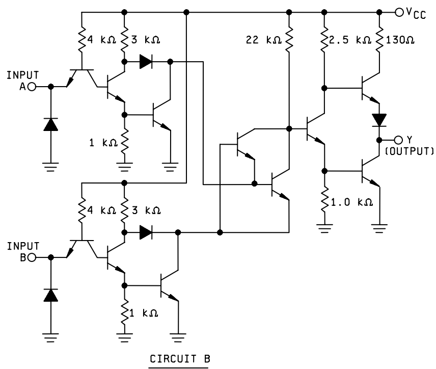
FIGURE 3. Schematic circuits.
