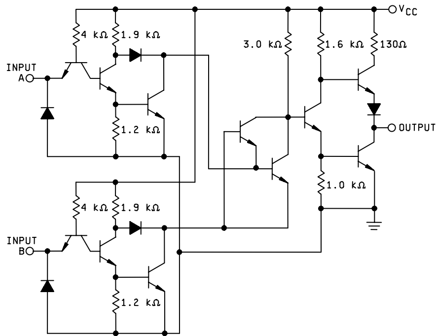
CIRCUIT C
