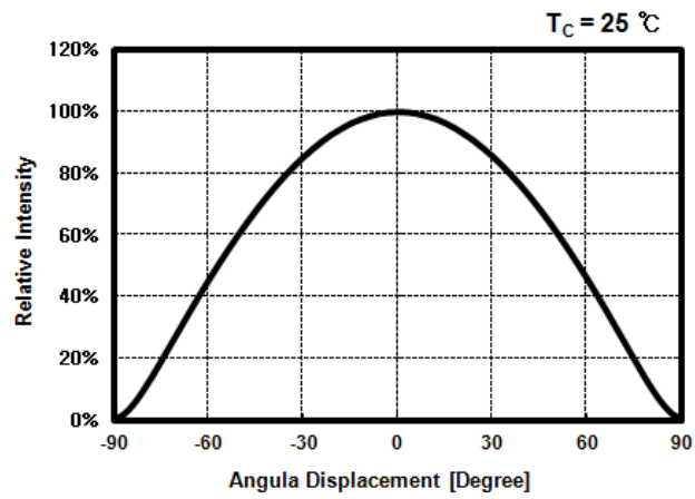
Radiation Pattern
