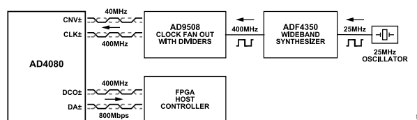
Figure 48. Single Lane, LVDS Data Interface Clocking Example
