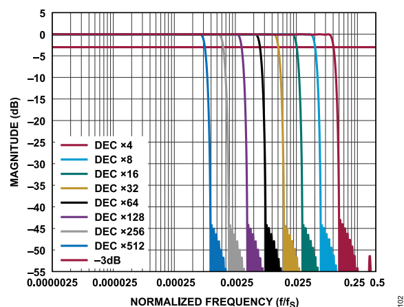
Figure 107. Sinc5 + Compensation Filter Response
