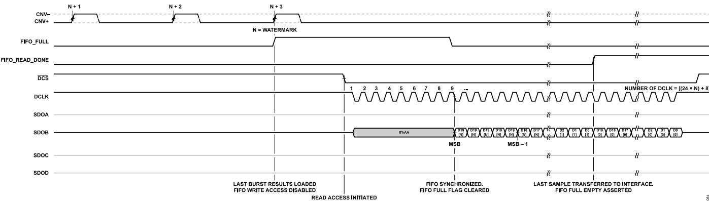
Figure 87. Asynchronous Capture Read Timing, Data FIFO Enabled, Single Data Lane
