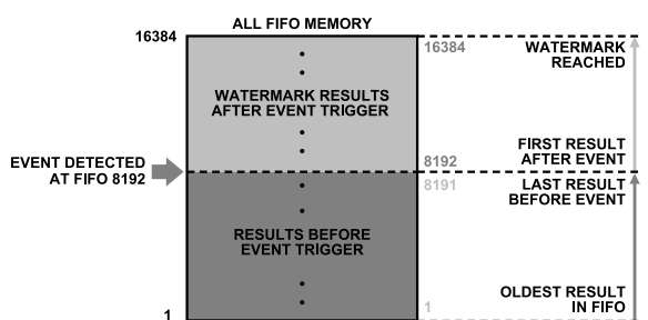
Figure 94. FIFO Event Capture Mode Read All FIFO Mode Example, Locating Event Position in FIFO
