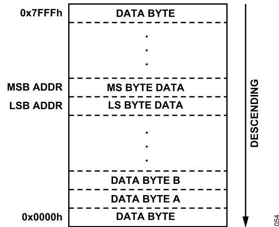
Figure 57. Generic Byte Wide Memory, Multibyte Register Example
