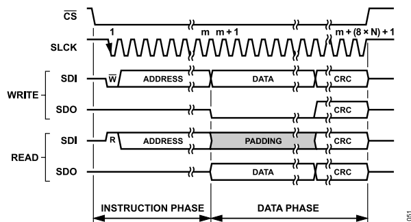
Figure 54. Generic SPI Configuration Write Operation, CRC Enabled
