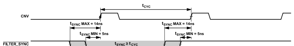
Figure 98. Filter Reset Timing
