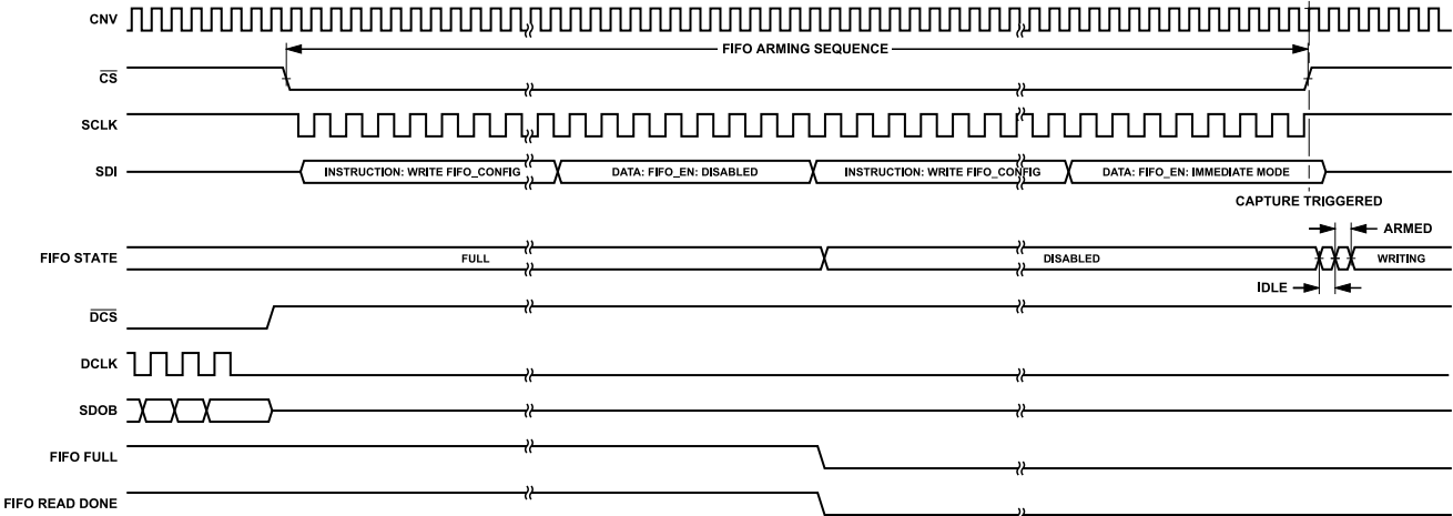
Figure 91. Immediate Trigger Mode Rearming
