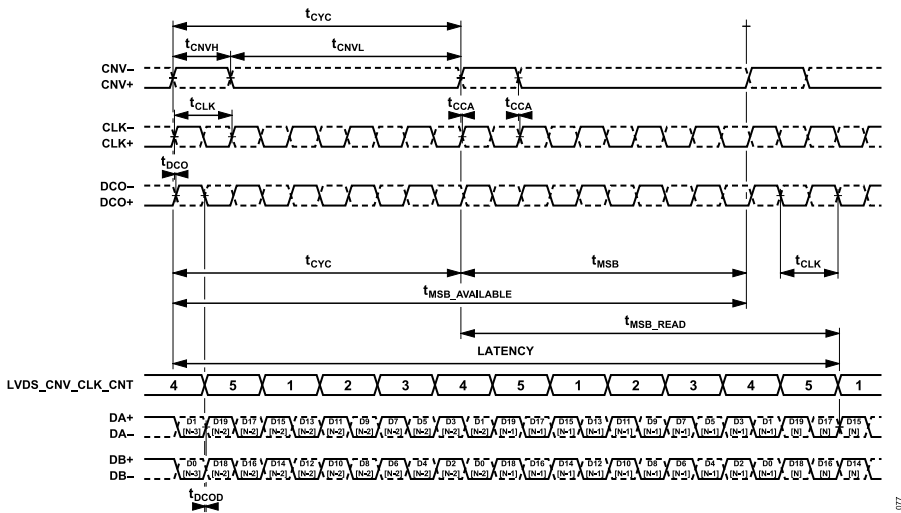
Figure 80. Dual Lane LVDS, Echo Clock Mode, LVDS_CNV_CLK_CNT Position Example
