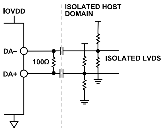
Figure 78. Isolated LVDS
