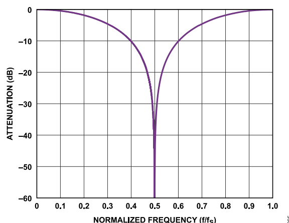
Figure 100. Sinc1 Filter Response, Decimate by 2
