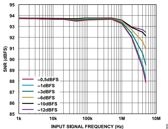
Figure 5. SNR vs. Input Signal Frequency (Amplitude = -0.5 dBFS, -1 dBFS, -3 dBFS, -6 dBFS, -10 dBFS, and -12 dBFS)
