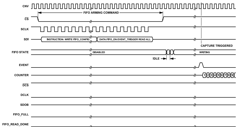
Figure 95. Event Trigger Capture Mode, Read All FIFO Rearming
