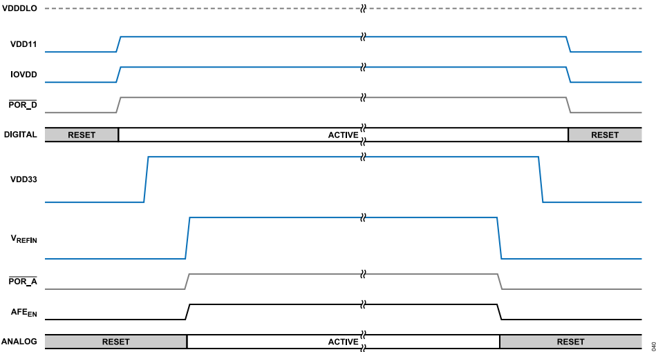
Figure 42. Power Supply Sequence, Externally Generated IOVDD, VDD11
