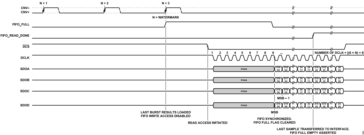
Figure 88. Asynchronous Capture Read Timing, Data FIFO Enabled, Quad Data Lane Configuration
