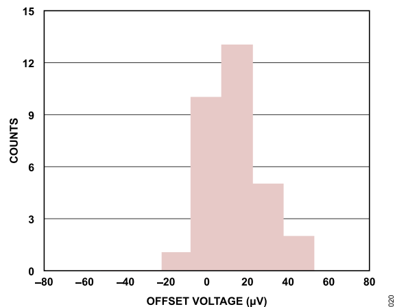
Figure 20. Offset Voltage Histogram
