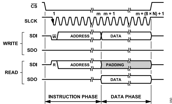
Figure 53. Generic SPI Configuration Frame, CRC Disabled
