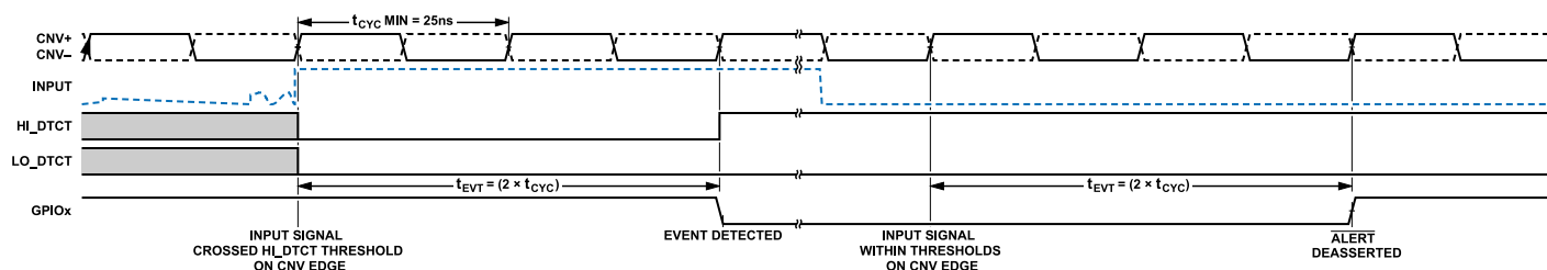
Figure 83. Event Detection Timing
