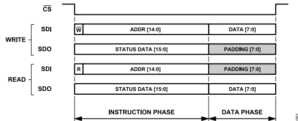
Figure 65. Long Instruction Mode, Data Status Enabled, CRC not Enabled
