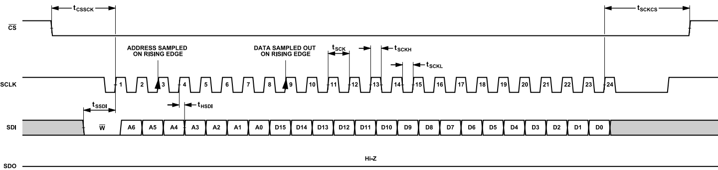
Figure 69. Configuration SPI Timing, Data Write Frame, 8-Bit Instruction Mode, Streaming Mode, Multibyte Register
