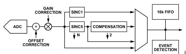
Figure 96. Digital Filter Selection Options
