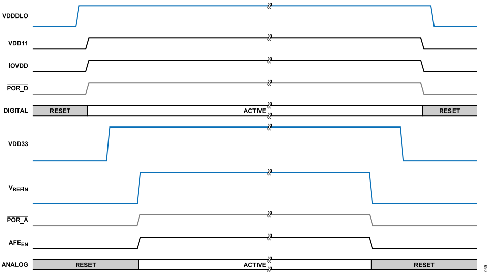
Figure 41. Power Supply Sequence, Internally Generated IOVDD, VDD11
