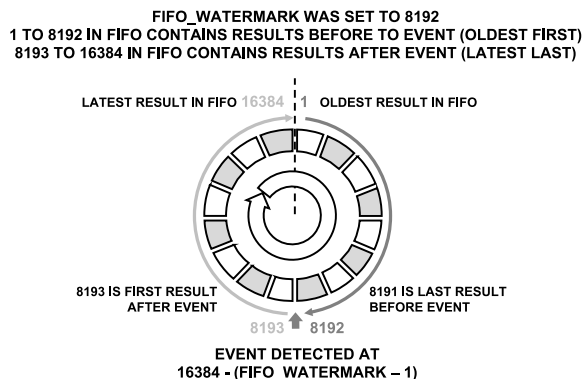
Figure 93. Event Capture Mode Read All FIFO Mode Example, FIFO Filling
