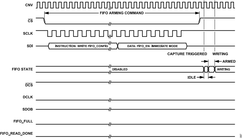
Figure 90. Immediate Trigger Mode Arming
