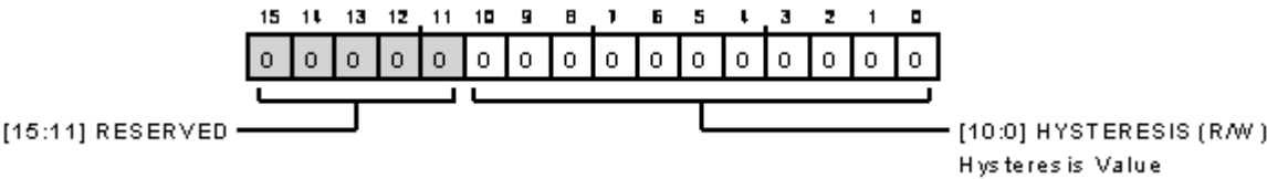
Figure 135. Event Detection Hysteresis Configuration Register
