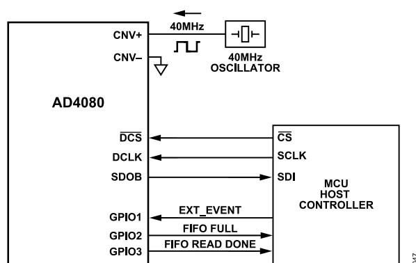
Figure 50. SPI Data Interface Clocking Example
