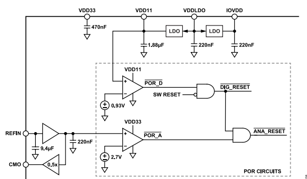
Figure 40. Simplified Diagram of POR Circuit
