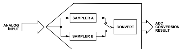
Figure 31. Simplified Representation of the AD4080 SAR ADC
