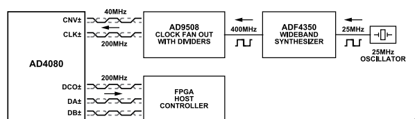
Figure 49. Dual Lane, LVDS Data Interface Clocking Example
