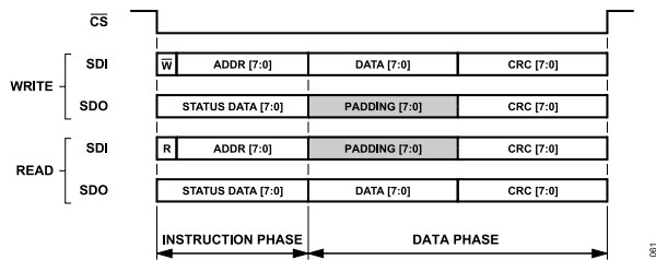
Figure 64. Short Instruction Mode, Data Status Enabled, CRC Enabled
