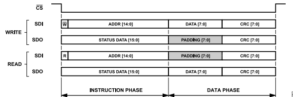
Figure 66. Long Instruction Mode, Data Status Enabled, CRC Enabled
