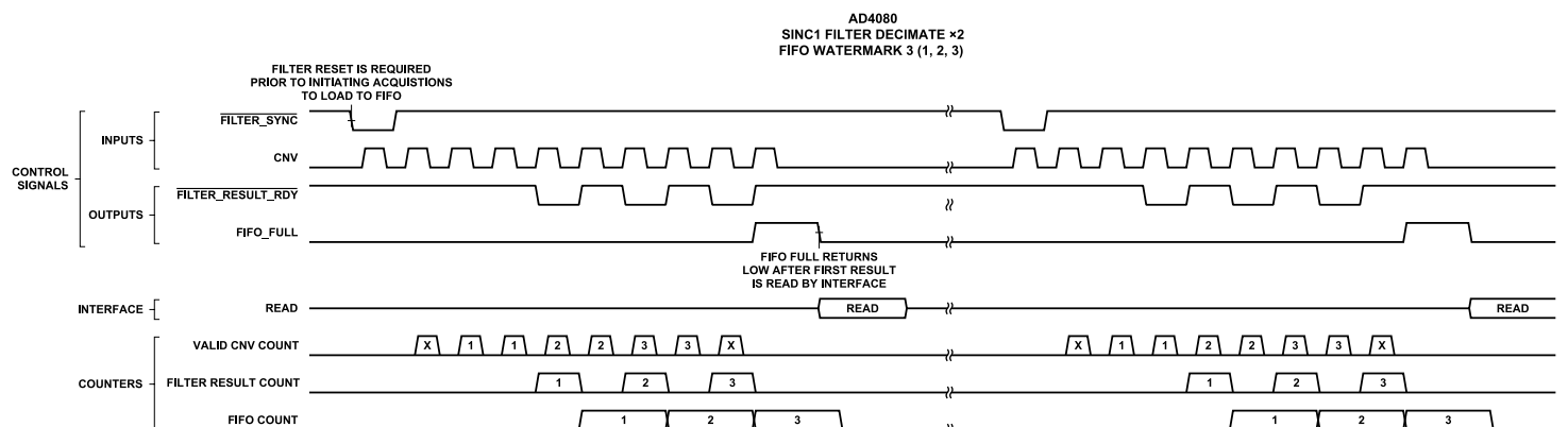
Figure 99. Description of Filter Timing with FIFO
