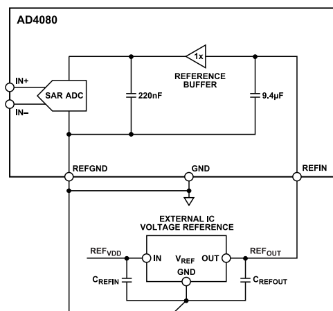
Figure 47. AD4080 General External Reference Design Functional Diagram
