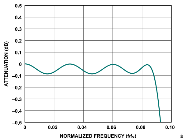
Figure 106. Sinc5 + Compensation Filter Response, Decimate by 2, Pass-Band Ripple
