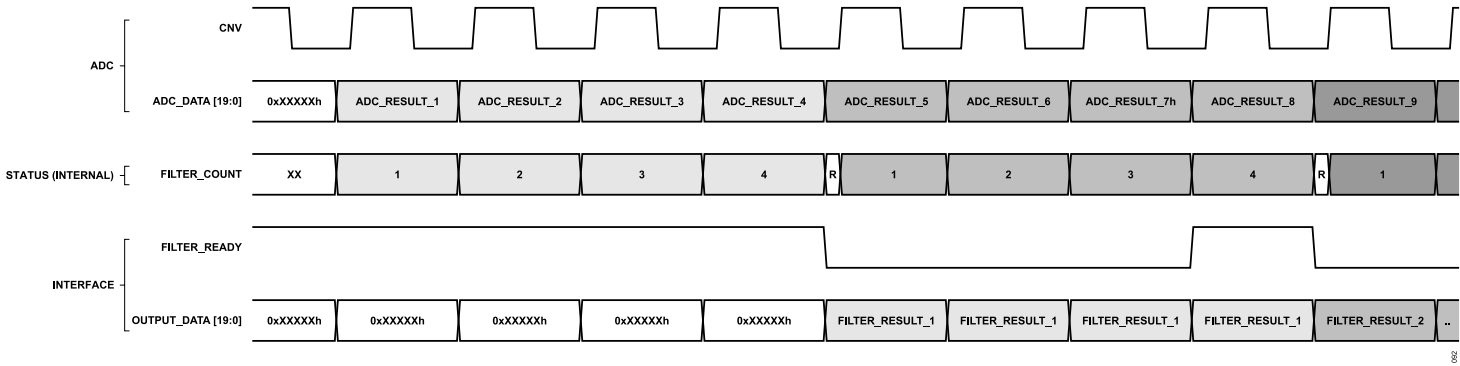
Figure 97. Digital Filter Decimate by 4 Frame Overview
