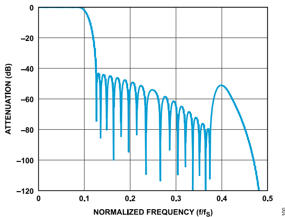
Figure 105. Sinc5 + Compensation Filter Response, Decimate by 2
