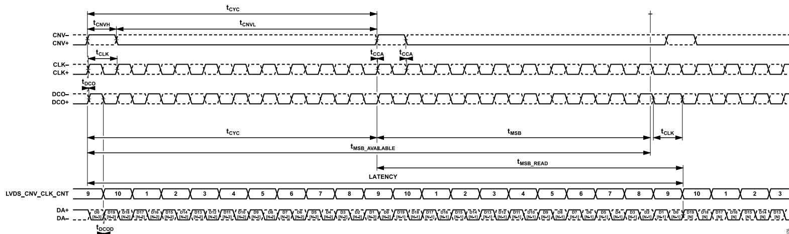
Figure 79. Single Lane LVDS, Echo Clock Mode, LVDS_CNV_CLK_CNT Position Example
