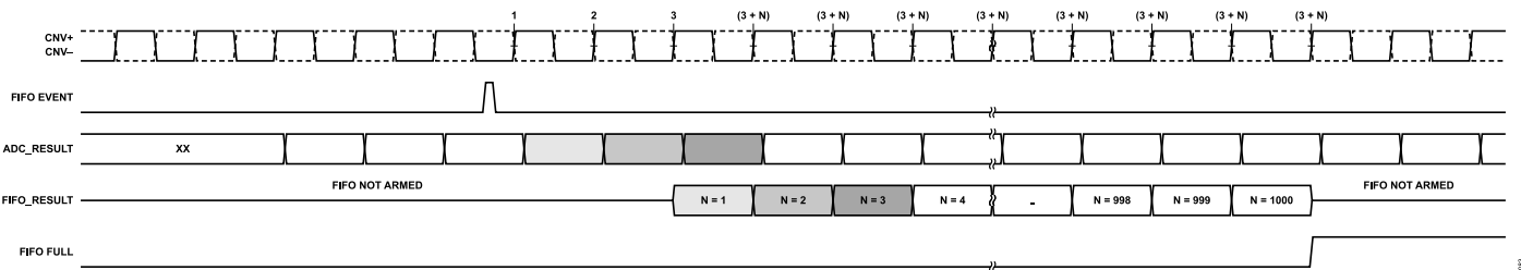
Figure 86. FIFO Data Capture Example, WATERMARK = 1000
