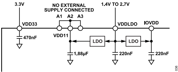
Figure 38. Internally Regulated (1.1V) Supply Configuration
