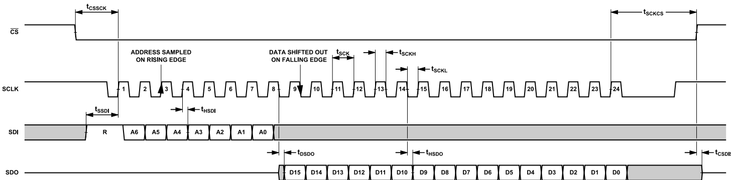
Figure 72. Configuration SPI Timing, Data Read Frame, 8-Bit Instruction Mode, Steaming Mode, Multibyte Register
