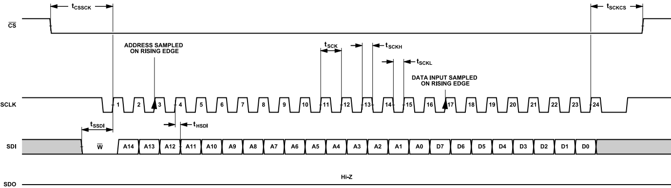
Figure 67. Configuration SPI Timing, Data Write Frame, 16-Bit Instruction Mode (Default)
