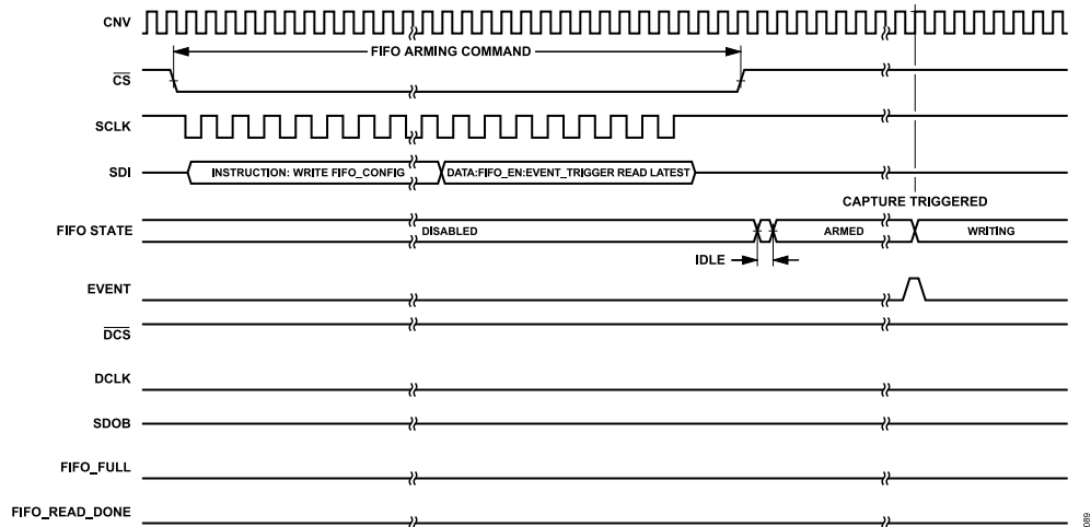
Figure 92. Event Triggered Capture, Read Latest WATERMARK Arming
