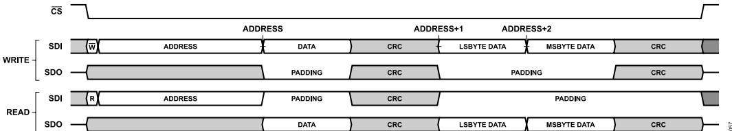
Figure 60. Streaming Mode Configuration with CRC Enabled, ADDR_ASCENSION = 1
