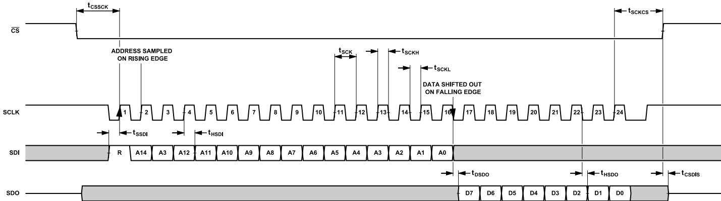
Figure 70. Configuration SPI Timing, Data Read Frame, 16-Bit Instruction Mode (Default)
