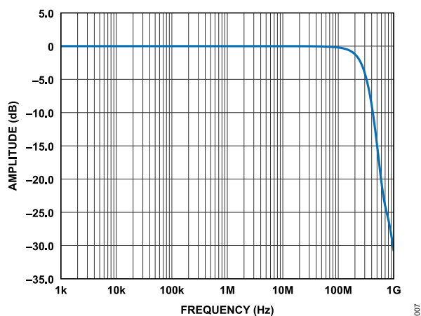
Figure 7. Small Signal -3 dB Bandwidth at 40 MSPS
