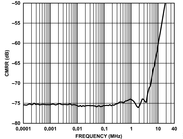
Figure 30. AC CMRR vs. Input Frequency
