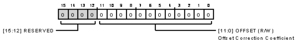
Figure 138. Offset Correction Register
