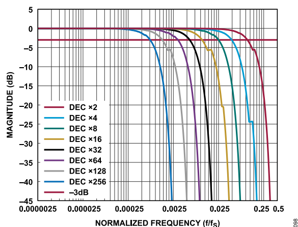
Figure 104. Sinc5 Filter Response, All Decimation Rates
