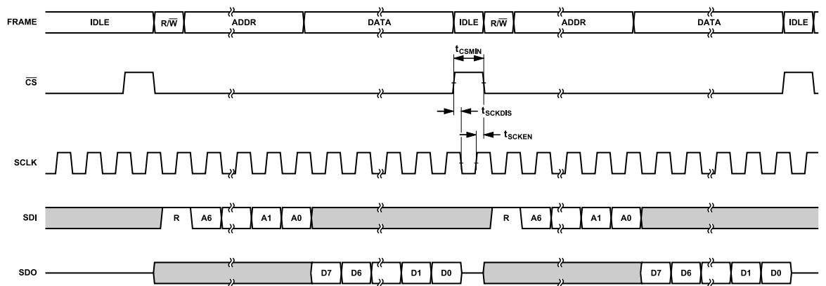
Figure 73. Configuration SPI Timing, Data Read Frame, Continuous SCLK
