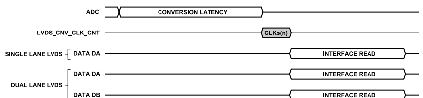
Figure 81. LVDS Data Transfer Latency
