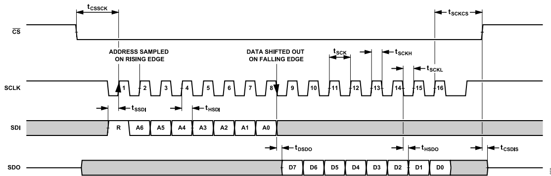
Figure 71. Configuration SPI Timing, Data Read Frame, 8-Bit Instruction Mode
