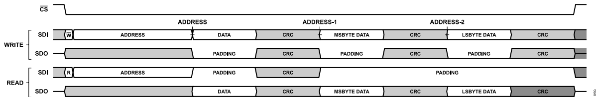
Figure 62. Streaming Mode Configuration with CRC Enabled, STRICT_REGISTER_ACCESS = 0 (Disabled), ADDR_ASCENSION = 0
