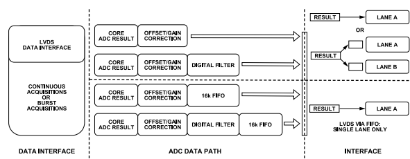
Figure 51. LVDS Data Interface Options
