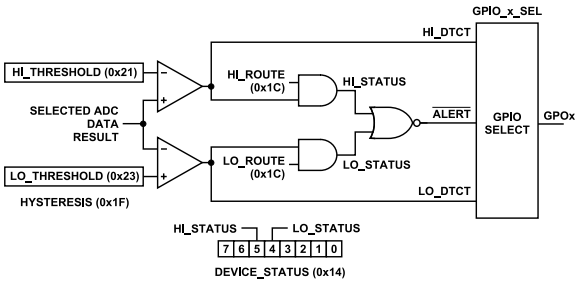
Figure 82. Internally Generated Event Detection Signal Path
