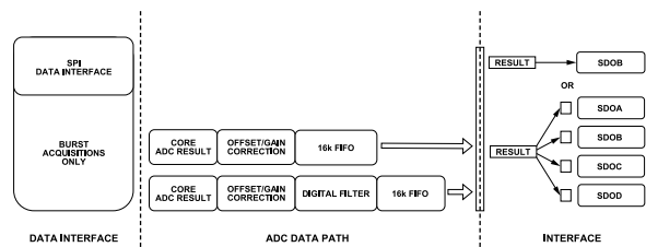
Figure 52. SPI Data Interface Data Path Options
