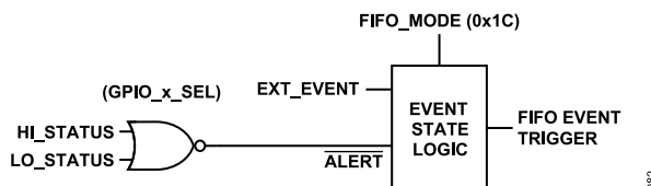
Figure 85. FIFO Event Detection Logic
