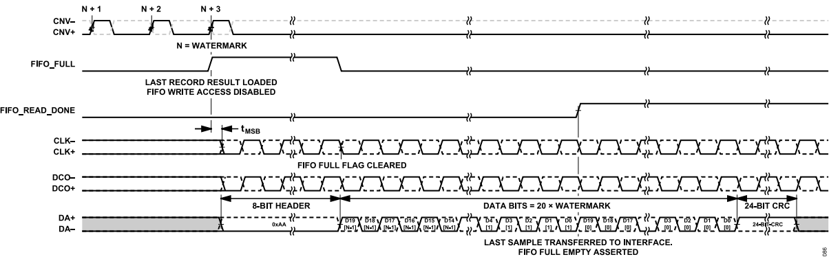
Figure 89. Asynchronous Capture Read Timing, Data FIFO Enabled, LVDS Configuration
