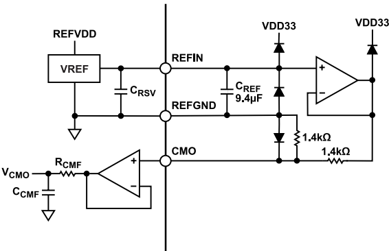
Figure 36. REFIN and CMO Internal Equivalent Circuit and Typical Application
