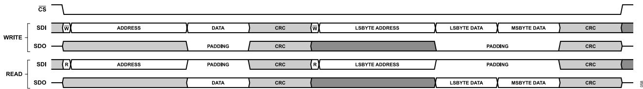
Figure 61. Single Instruction Mode Configuration with CRC Enabled, ADDR_ASCENSION = 1
