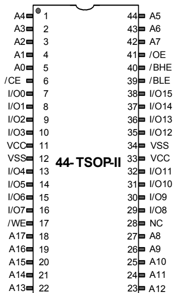
Figure 3. 44-pin TSOP II pinout (Single Chip Enable without ERR) – CY62146G/CY62146GSL [7]
