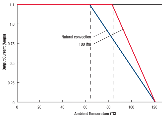
ULE-53/1.1-D48 Maximum Current Temperature Derating at sea level
