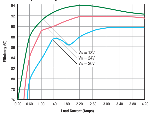
ULE-12/4.2-D24 Efficiency vs. Line Voltage and Load Current @25°C
