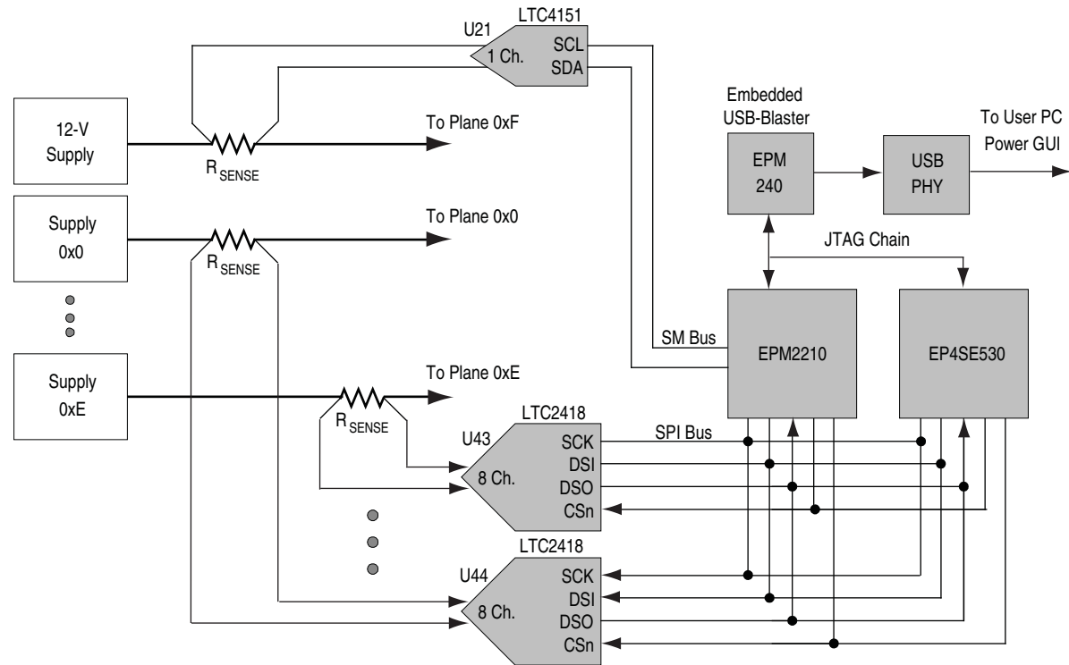
Figure 2-10. Power Measurement Circuit
