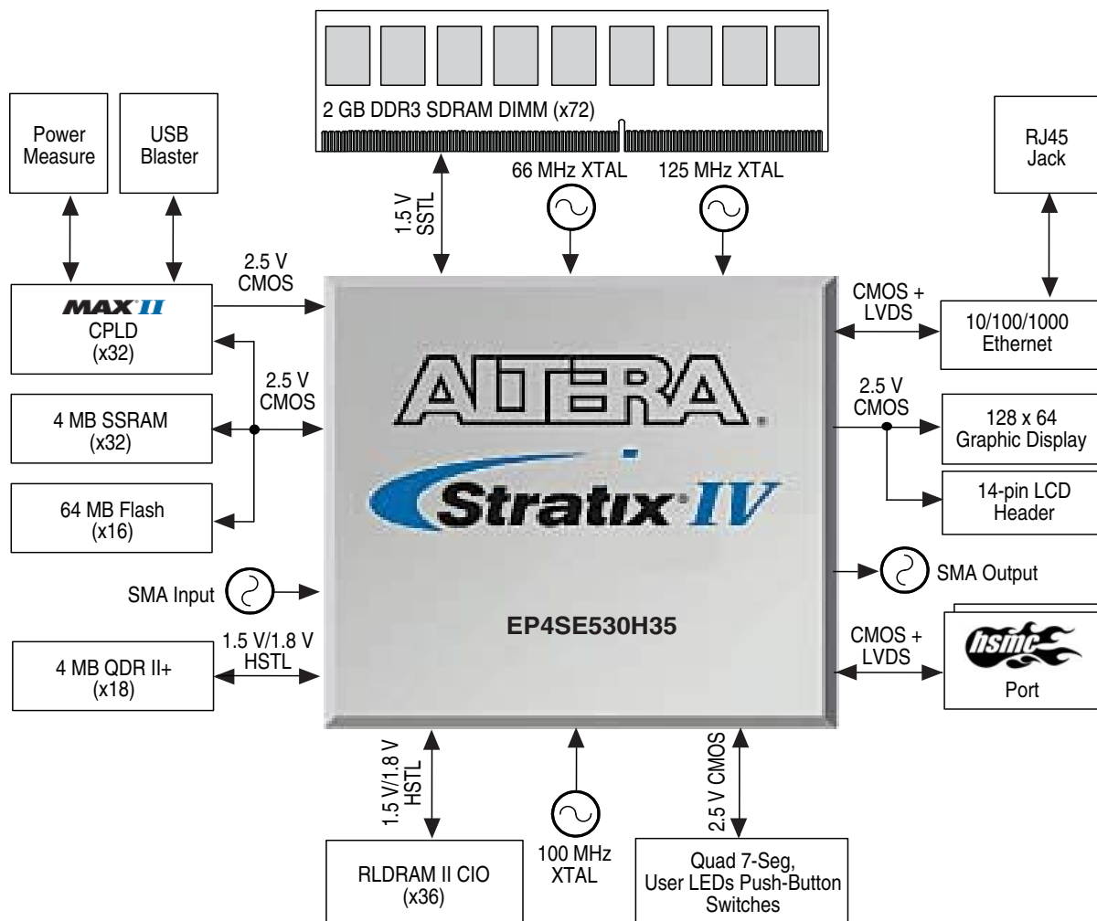
Figure 1–1. Stratix IV E FPGA Development Board Block Diagram
