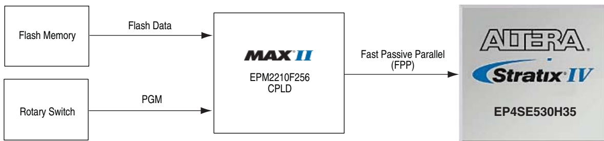
Figure 2-5. FPGA Programming from Flash Memory
