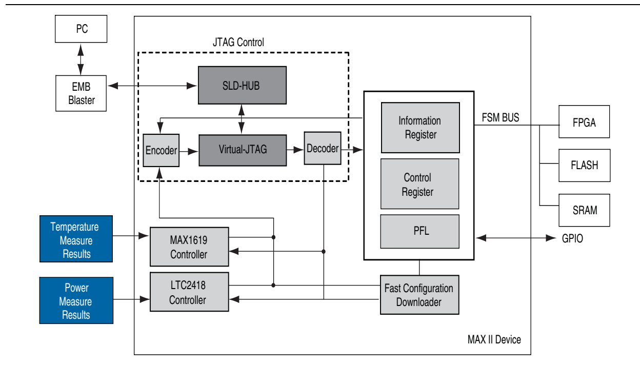
Figure 2-3. MAX II CPLD EPM2210 System Controller Block Diagram
