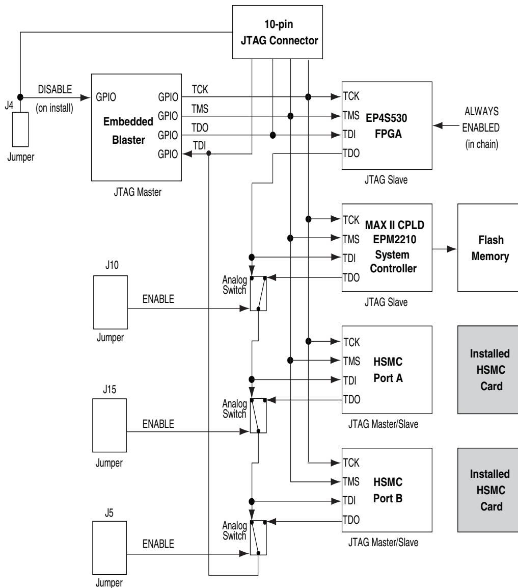
Figure 2-4. JTAG Chain
