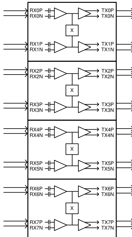
Figure 3. Block diagram showing all four 2x2 cross-points in the DS280MB810
