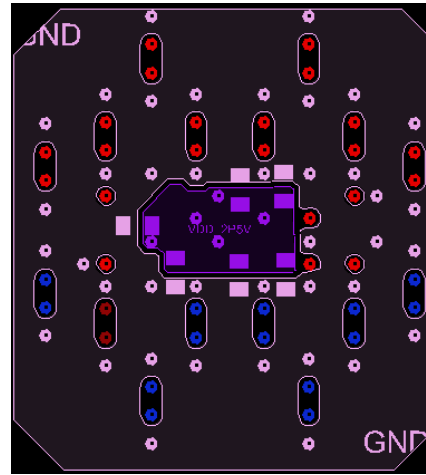
Figure 31. Stripline example, Bottom Layer
