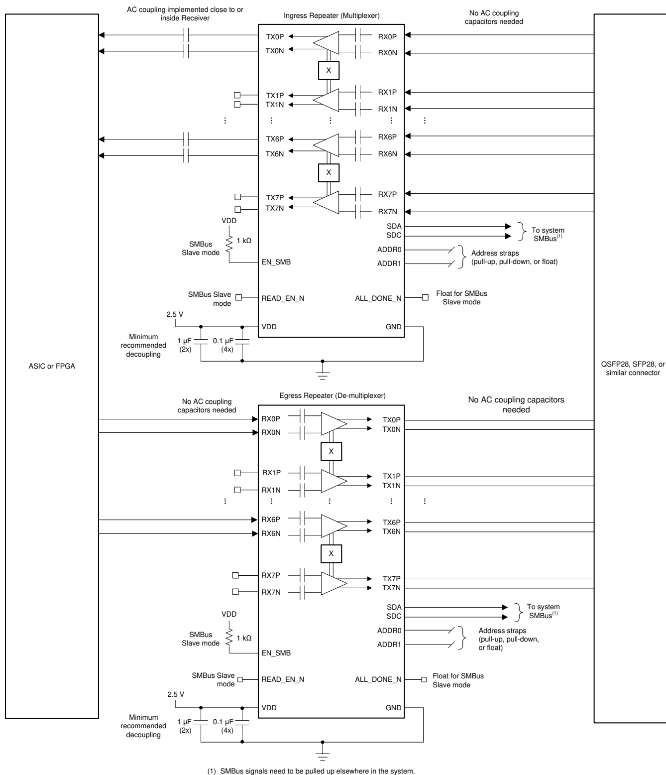
Figure 15. Front-port application simplified schematic
