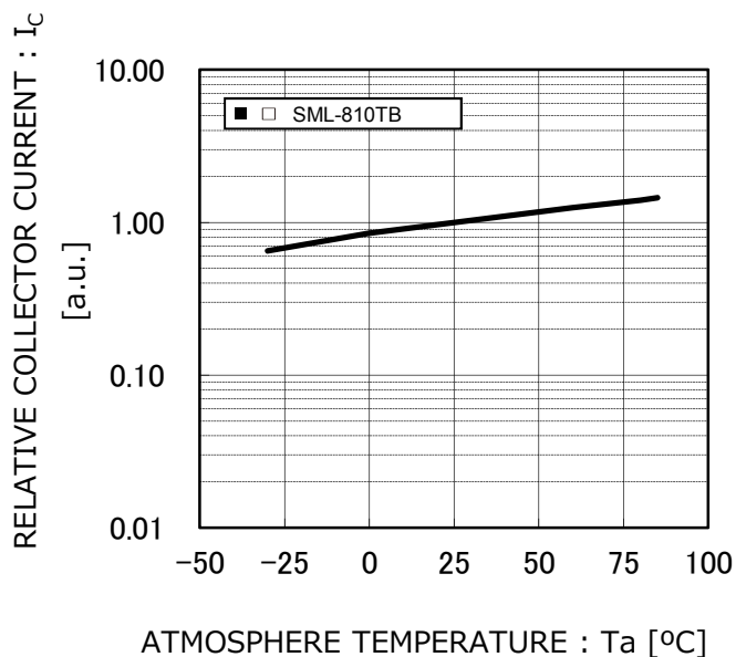
Fig.2 Relative Collector Current - Ambient Temperature
