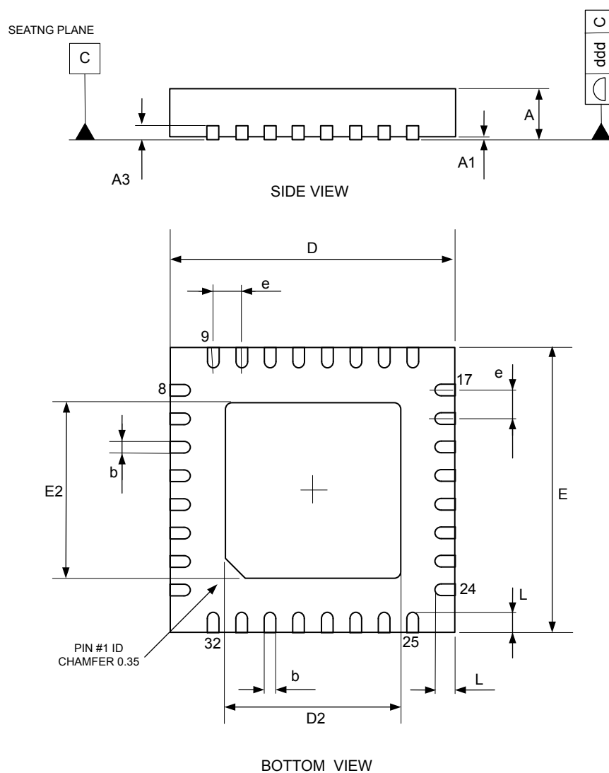
Figure 19. VFQFPN32 - Outline
