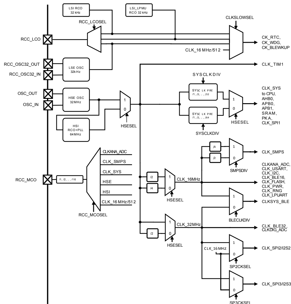
Figure 6. Clock tree
