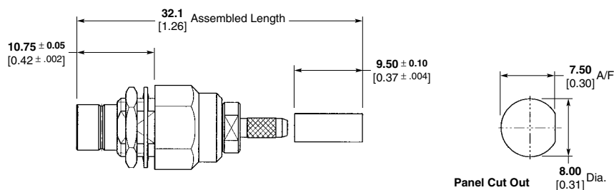
Panel Cut Out
