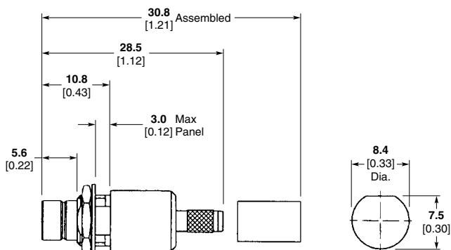
Mounting Detail
