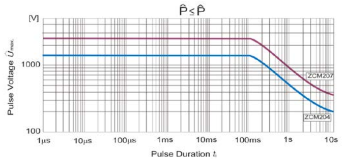
Pulse Voltage
