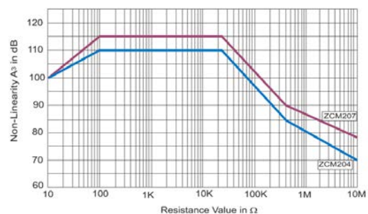
Non- Linearity
