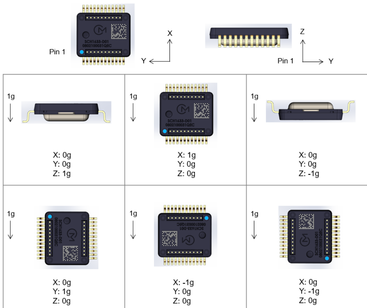
Figure 3 SCH16T series measurement directions for gyroscope and accelerometer. Output is showing positive value when component is moved in the direction of the arrow.
