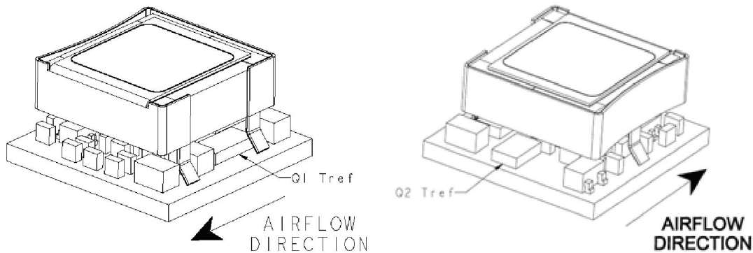
Preferred airflow direction and location of hot-spots of the module ( T_{ref} ).
