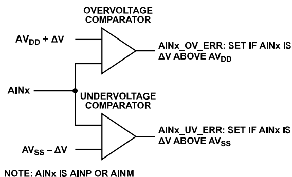
Figure 99. Analog Input Overvoltage/Undervoltage Monitors
