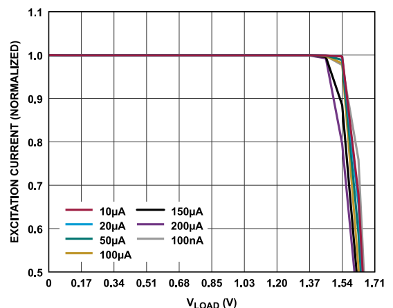
Figure 63. Output Compliance for Various IEXC Sources ( AV_{DD} = 1.71 V)
