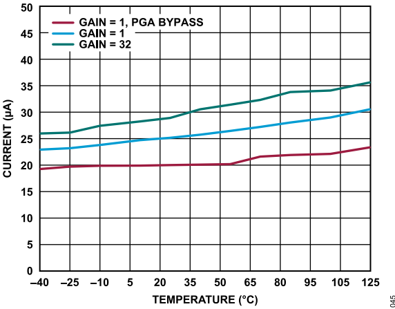
Figure 46. AV_{DD} Current vs. Temperature for Various Gains
