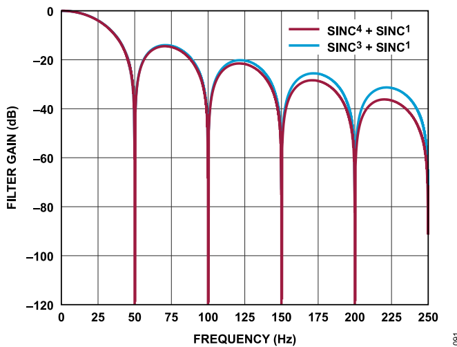
Figure 92. \text{Sinc}^3 + \text{Sinc}^1 and \text{Sinc}^4 + \text{Sinc}^1 Filter Response (FS = 6)
