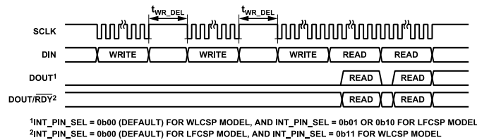
Figure 4. Delay Between Consecutive Serial Operations, 3-Wire Mode (CSB_EN Bit Set to 0), \overline{CS} Pin Connected Low
