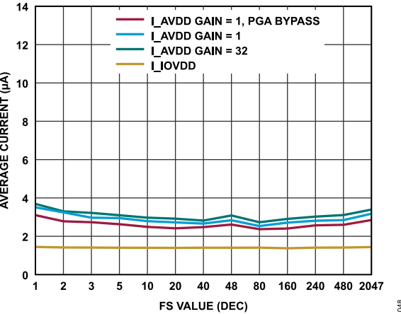
Figure 49. Duty-Cycling Current Consumption ( AV_{DD} and IOV_{DD} ), DUTY\_CYC\_RATIO = 1/16
