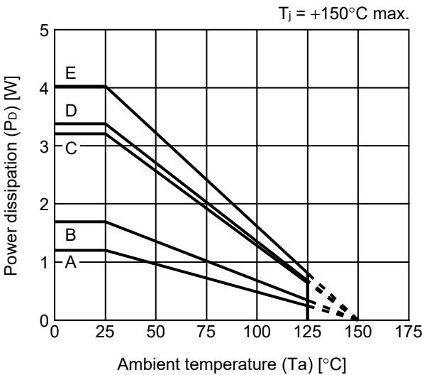
HSOP-8A
