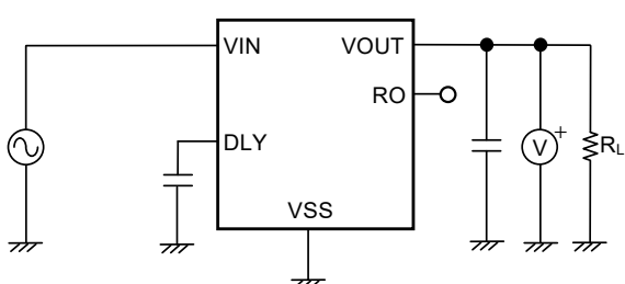
Figure 8 Test Circuit 3
