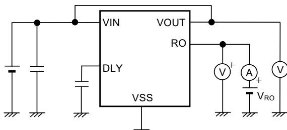
Figure 10 Test Circuit 5
