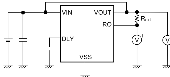
Figure 9 Test Circuit 4
