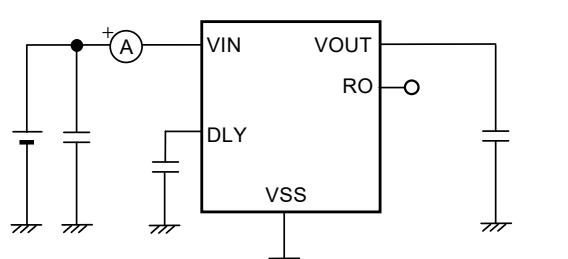
Figure 11 Test Circuit 6
