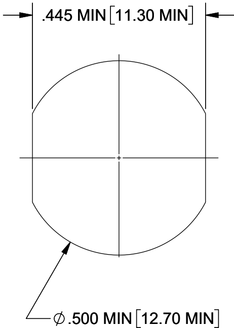
RECOMMENDED MOUNTING HOLE
