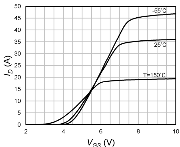
Fig.5 Transfer Characteristics
