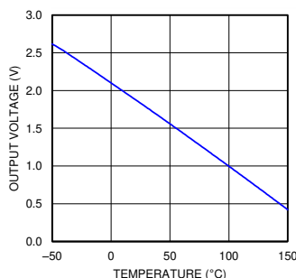
Figure 8-2. Analog Output Transfer Function
