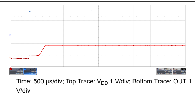
Figure 8-5. Output Turnon Response Time With a 1.1-nF Capacitive Load and V_{\text{DD}} = 3.3 \text{ V}
