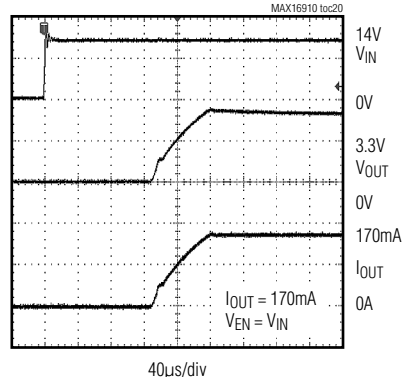
POWER-UP RESPONSE
