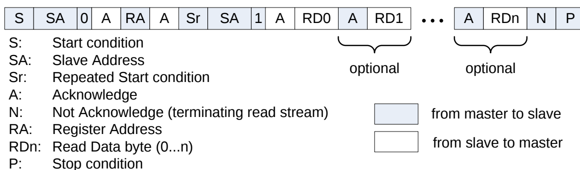
Figure 56 I2C read
