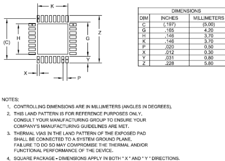
Figure 70 Land Pattern
