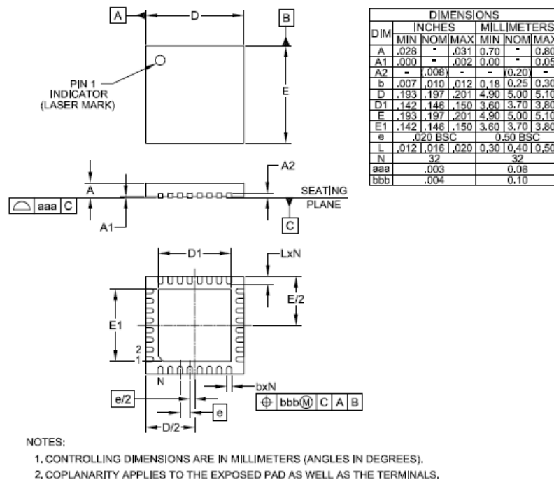
Figure 69 Package Outline Drawing
