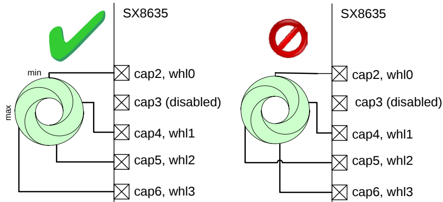
Figure 48 Button and Wheel good/bad configuration examples (II)
