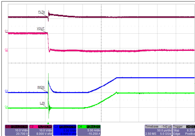
Figure 63. Hot Short: Fast Trip and Current Regulation
