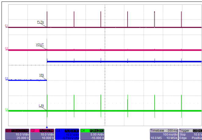
Figure 65. Hot Plug-In with Short on Output: Auto-Retry - TPS25940-Q1
