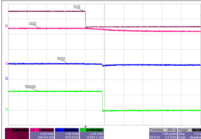
Figure 67. Power Good Response During Turn-OFF
