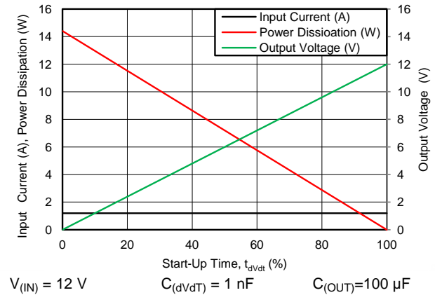
Figure 53. P_{D(INRUSH)} Due to Inrush Current
