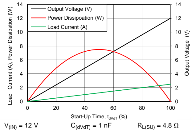
Figure 55. P_{D(LOAD)} in Load During Start-Up
