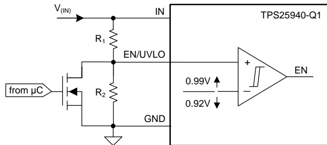
Figure 50. Shutdown Control
