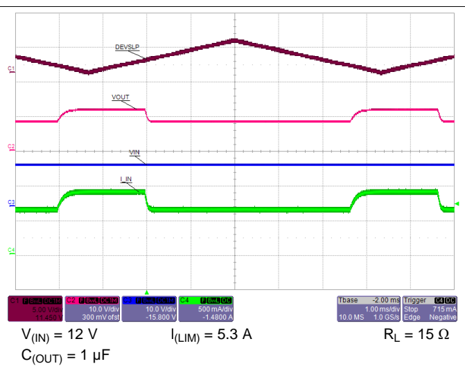
Figure 47. IN and OUT of DevSleep Mode with 800-mA Load. In DevSleep, Load Current gets Limited to I_{(\text{DEVSLP}(\text{LIM}))}
