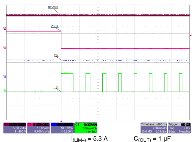
Figure 47. IN and OUT of DevSleep Mode with 800-mA Load. In DevSleep, Load Current gets Limited to I_{(\text{DEVSLP}(\text{LIM}))}
