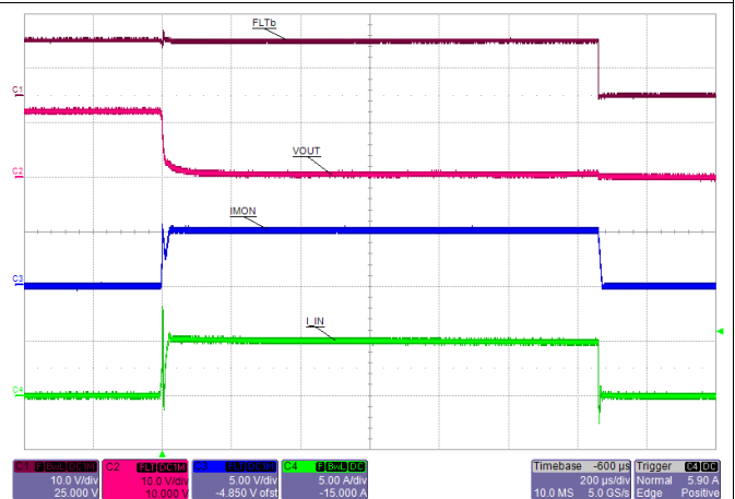
Figure 68. Hot Short: Latched - TPS25940L-Q1
