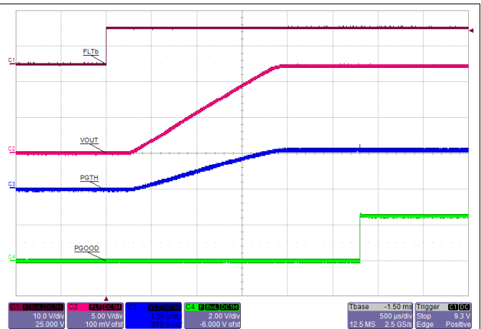
Figure 66. Power Good Response During Turn-ON
