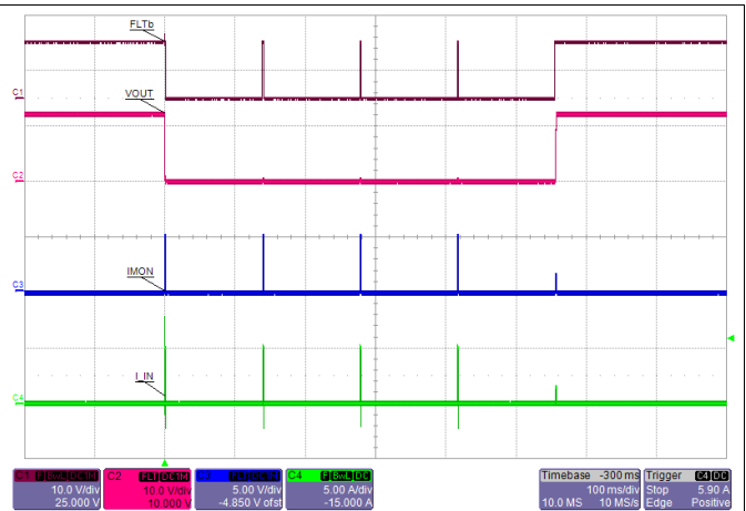
Figure 64. Hot Short: Auto-Retry and Recovery from Short Circuit - TPS25940-Q1
