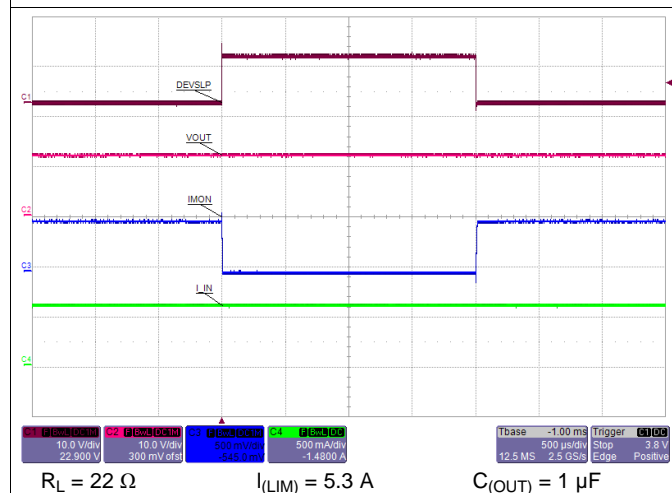
Figure 48. IMON Disabled in DevSleep Mode
