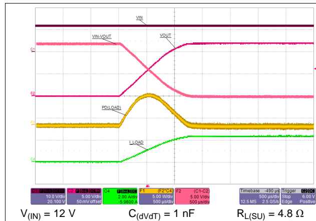
Figure 54. Start-Up With Load
