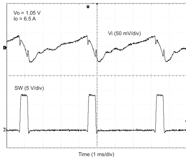
Figure 12-13. VOLTAGE RIPPLE AT INPUT ( I_O = 6.5\text{ A} )
