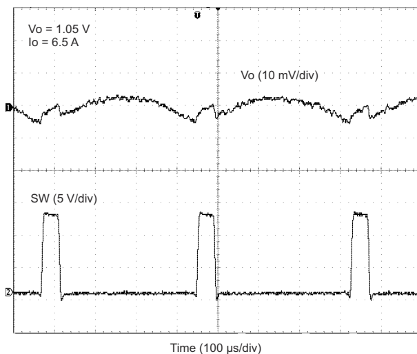
Figure 12-14. VOLTAGE RIPPLE AT OUTPUT ( I_O = 6.5\text{ A} )
