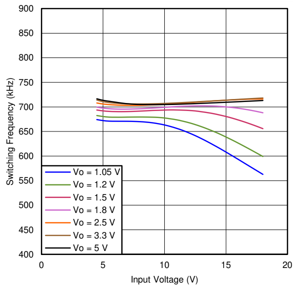
Figure 12-9. SWITCHING FREQUENCY vs INPUT VOLTAGE ( I_O = 1\text{ A} )
