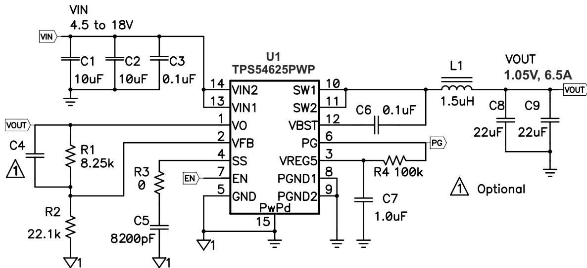
Figure 13-1. Schematic
