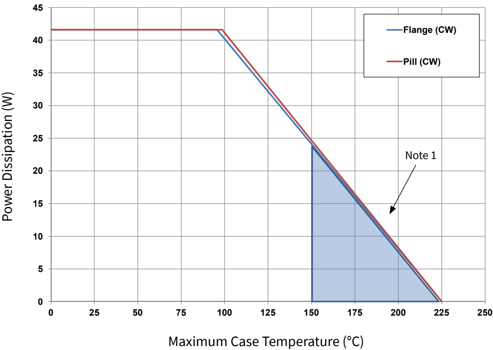
Figure 4. Transient Power Dissipation De-Rating Curve
