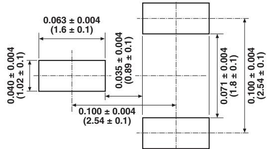
FIGURE 3 - RECOMMENDED LAND
