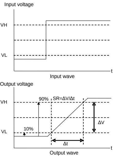
Figure 50. Slew rate input output wave
