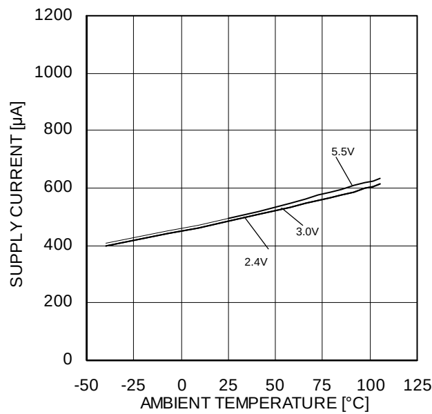
Figure 5. Supply Current – Ambient Temperature
