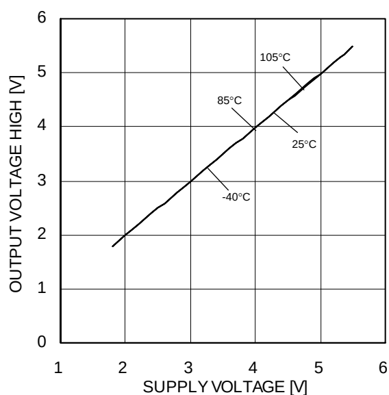
Figure 6. Maximum Output Voltage High – Supply Voltage ( R_L=10k\Omega )
