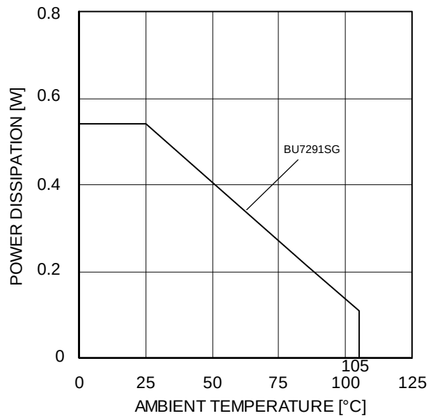
Figure 3. Derating curve
