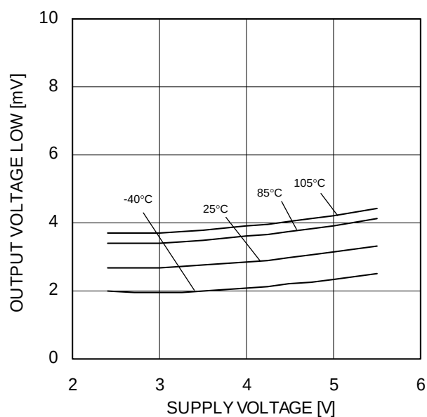
Figure 8. Maximum Output Voltage Low - Supply Voltage ( R_L=10k\Omega )
