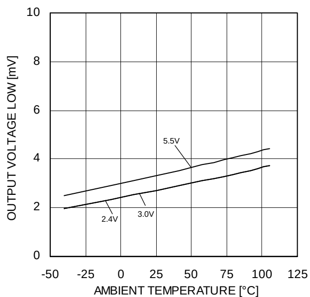
Figure 9. Maximum Output Voltage Low – Ambient Temperature ( R_L=10k\Omega )
