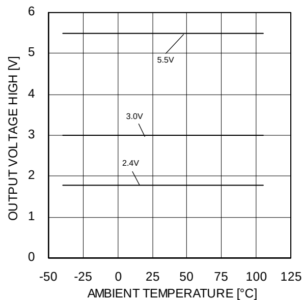
Figure 7. Maximum Output Voltage High – Ambient Temperature ( R_L=10k\Omega )
