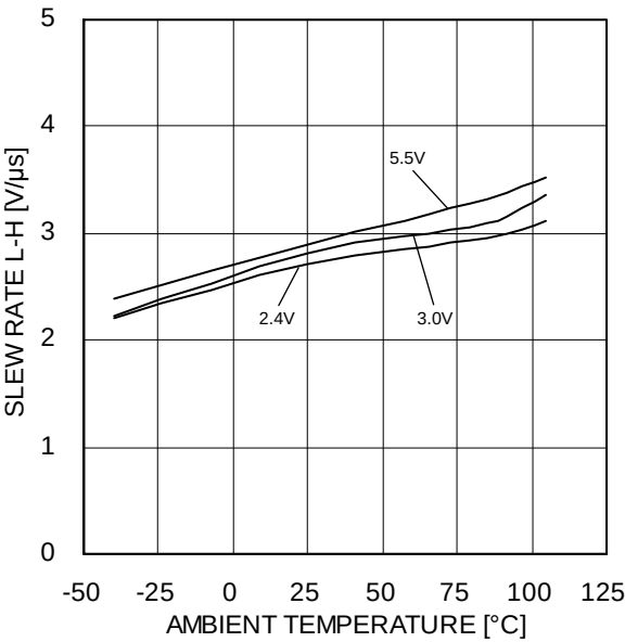
Figure 22. Slew Rate L-H – Ambient Temperature
