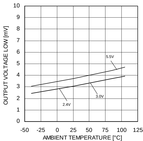
Figure 32. Maximum Output Voltage Low – Ambient Temperature ( R_L=10k\Omega )
