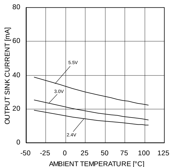
Figure 13. Output Sink Current – Ambient Temperature (OUT=VSS+0.4V)
