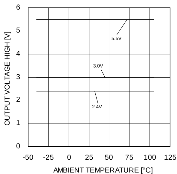
Figure 30. Maximum Output Voltage High – Ambient Temperature ( R_L=10k\Omega )
