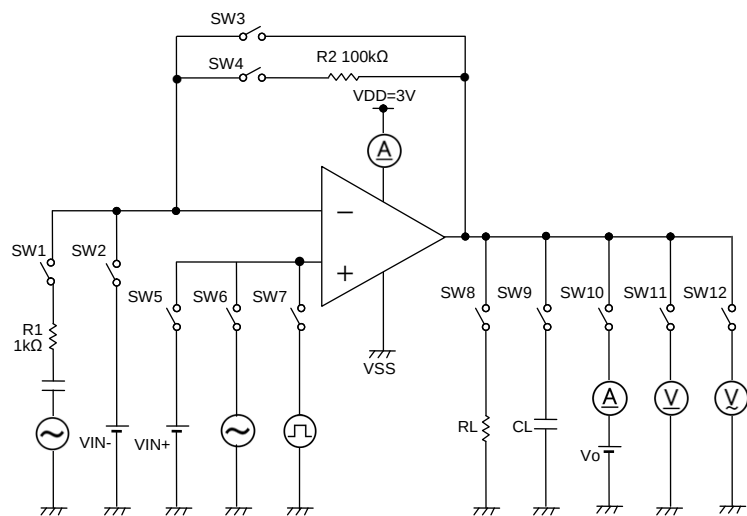
Figure 49. Test circuit 2
