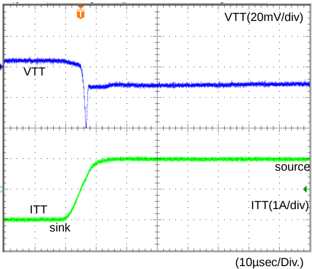
Figure 6. DDR1 (1A→-1A)
