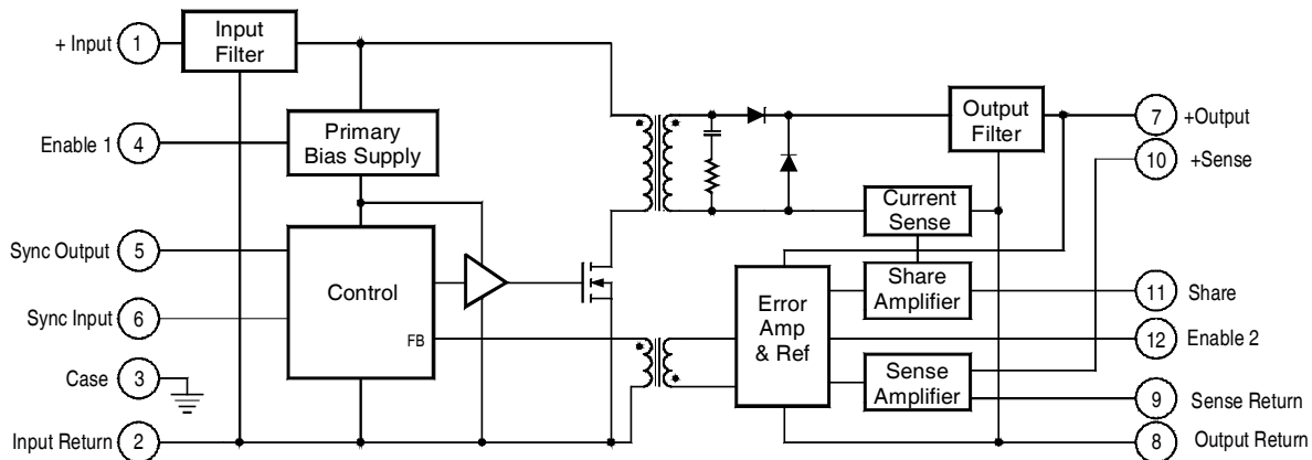
Figure 1. Single Output
