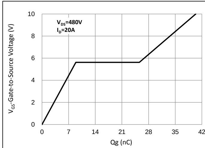
Fig.7 Gate-Charge Characteristics
